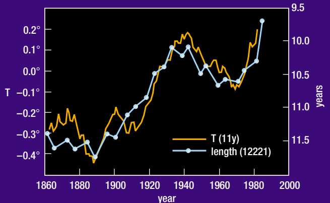
5: Eleven-year running mean of the annual average northern hemisphere land-air temperature relative to the average temperature 1951–1980 and the filtered length of the sunspot cycle. (From Friis-Christensen and Lassen 1994, by permission.)
