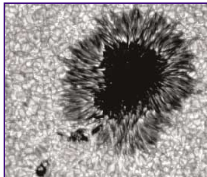
2: Image of a sunspot and the surrounding photosphere. The inner, darker part is called the umbra, the outer striated part is the penumbra. The sunspot is surrounded by granules, convection cells with a bright core harbouring hot upflows and dark boundaries (so-called intergranular lanes) composed of cool downflowing gas. (Figure kindly provided by T Berger, Lockheed-Martin Solar and Astrophys. Lab.)
