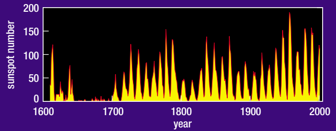
4: The yearly sunspot-number record since the beginning of telescopic observations. The period in the second half of the 17th century that was practically free of sunspots is called the Maunder minimum.
