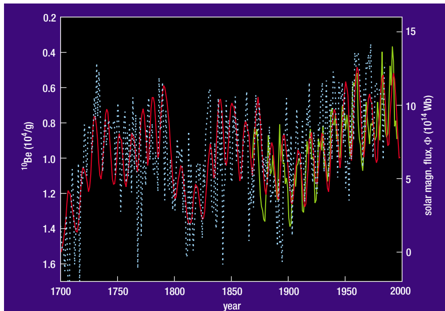
10: Evolution of the open magnetic flux at the solar surface since the end of the Maunder minimum in 1700. Model predictions by Solanki et al. (2000) are represented by the red curve, reconstructions by Lockwood et al. (1999) based on geomagnetic indices by the green curve and the ^{10}\text{Be} concentration in ice cores (corresponding to the inverted scale on the left y-axis, Beer et al. 1990) by the dotted curve.
