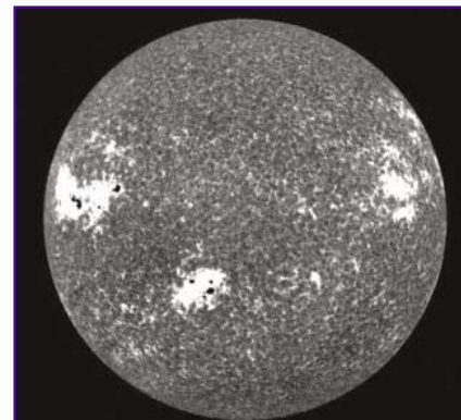
3: An image of the full solar disc taken in the light of singly ionized calcium. The dark features are sunspots, the bigger bright patches are faculae and the small bright features present all over the solar disc are network elements.
